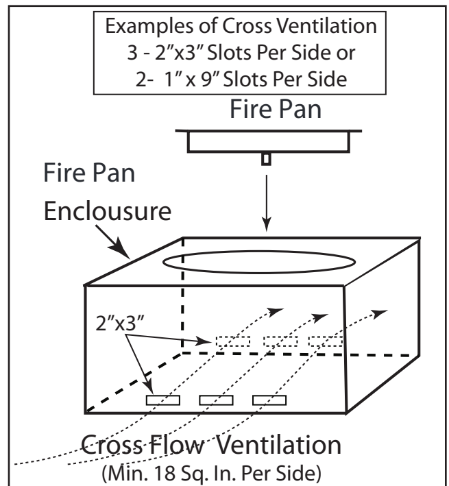
Figure 3. Cross Ventilation Example
