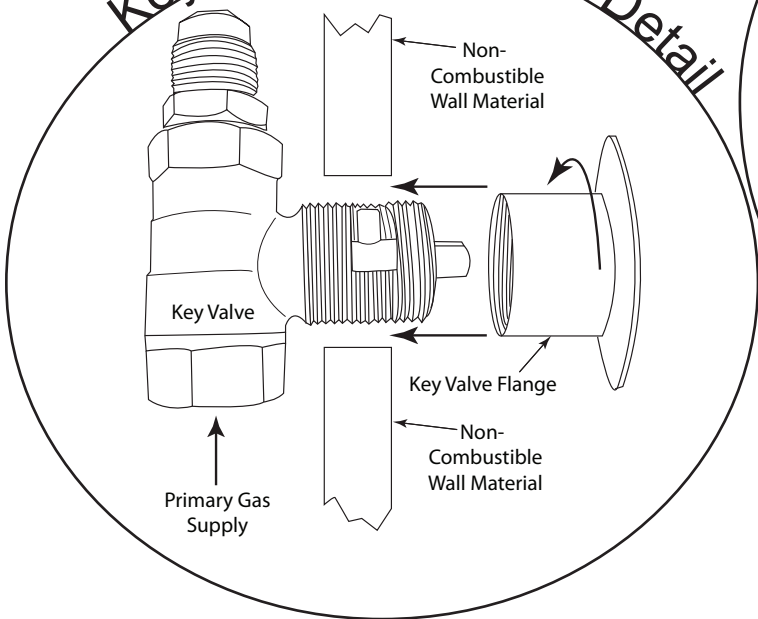
Fig. 5 Typical installation.
